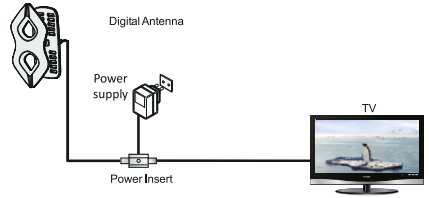
Installation 2 : Directly connected to HDTV(Fig.5)
