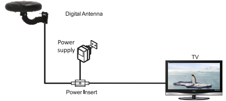
Installation 2: Directly connected to HDTV(Fig.5)
